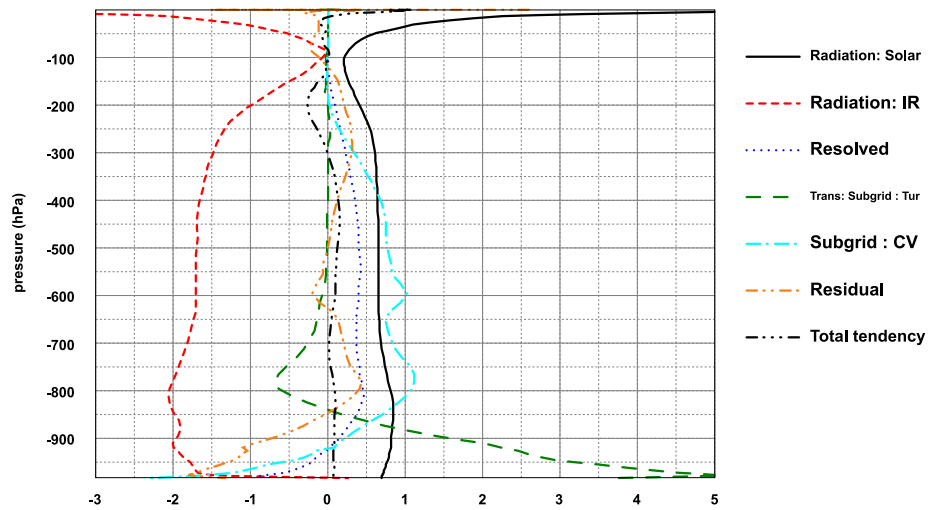
TEMPERATURE BUDGET (K/day) , OPER (20221122T0000P.DHFZOF CST+0072.lfa.mh) 2022-11-22 00:00 + 3 J, 1 dom., 105 niv.
