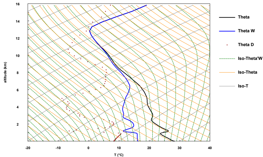
Tephigram, G6ZJ: potential temperature , lon= 1.38034 lat= 43.57835 Analysis Fri 6.10.2023 00h UTC + 16h, Valid Fri 6.10.2023 16h UTC (16:06 LST)
