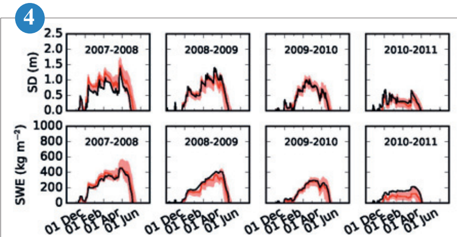
Snow depth (SD) and snow water equivalent (SWE) observed (in black) and simulated by 35 equiprobable members of the ESCROC system during 4 winter seasons from 2007 to 2011. The red envelope represents the uncertainty of the parameterizations in the snowpack model (difference between 5th and 95th percentiles of the ensemble) and the red line represents the ensemble median.
