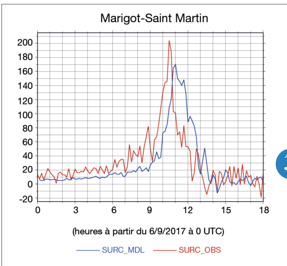
Comparison between the measured (red line) and the modelled (blue line) storm surge at Marigot (in the north of Saint Martin in the Lesser Antilles) during the Irma hurricane path, the 6th September 2017. The storm surges model is driven by the wind and the atmospheric pressure from the AROME model of Météo-France.
