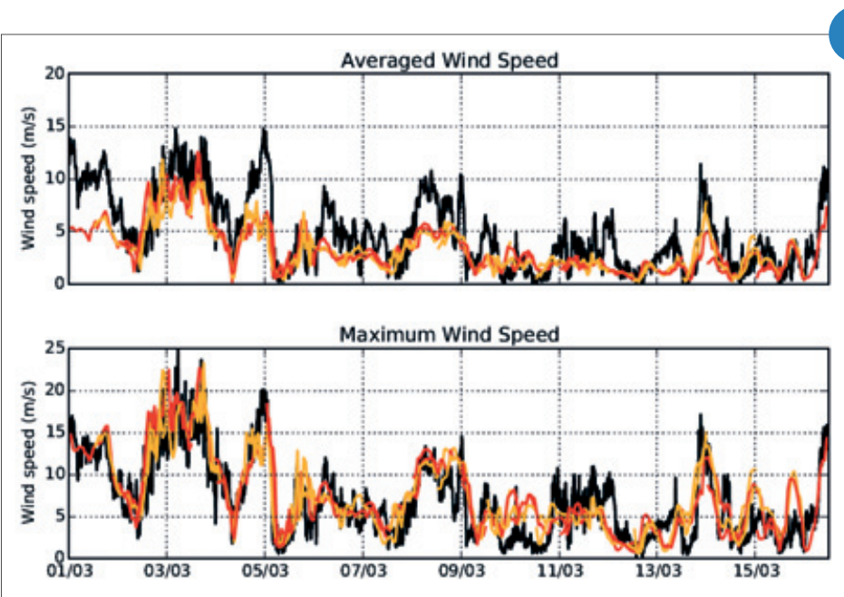
Mean (top) and maximum (bottom) wind speed at « Col du Lac Blanc »: Observations (black) and short range forecasts from AROME model (00h00 UTC: red; 12 h00 UTC: in orange) for the period ranging from March 1st to March 16th 2016.
