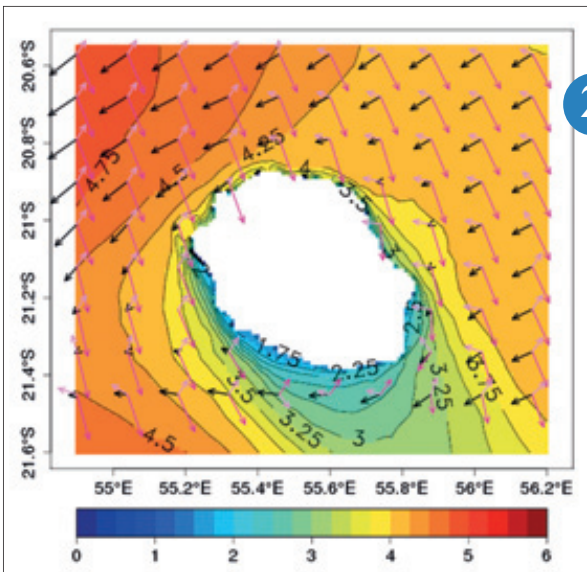
Significant wave height of the total sea (in meters) of WW3 on 31 January 2013 at 18:00 (UTC) in Reunion Island during Felleng hurricane (category 3) Dark violet arrows describe the direction of primary swell, light arrows the secondary swell and black arrows the wind sea.
