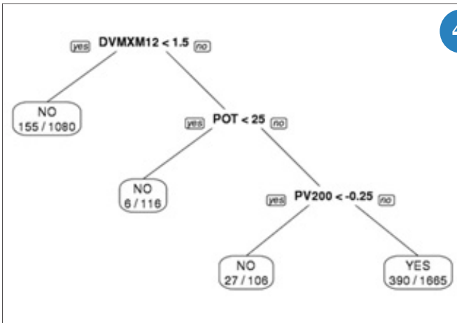
◀ The decision tree for the prediction of rapid intensification (class label YES) in the next 24 hours, based on the values of 3 predictors: DVMXM12 (the previous 12-h intensity change, in m/s), POT (the Maximum Potential Intensity MPI minus the initial intensity, in m/s), and PV200 (the 200-hPa potential vorticity averaged in a 200-800-km region surrounding the storm center, in PVU). The numbers in the leaf nodes indicate the misclassified samples and the total number of samples from both classes fulfilling the conditions of each tree path.
