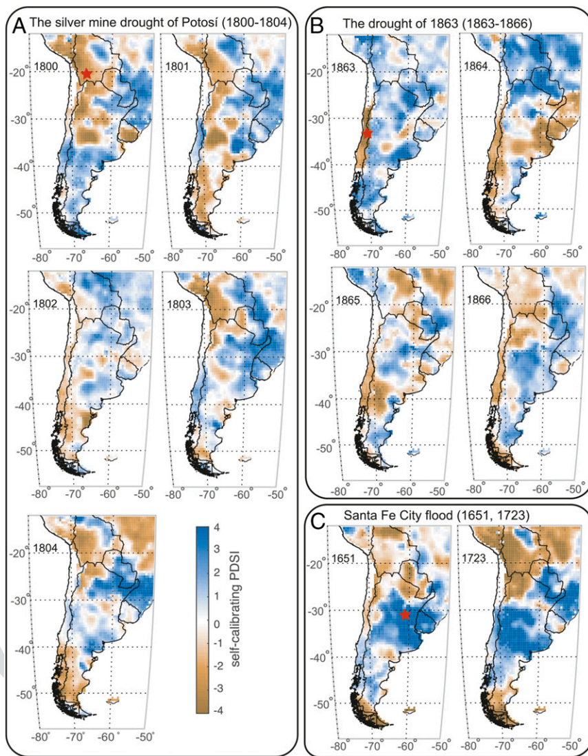
Fig. 3. Summer scPDSI maps of historical extremely dry and wet events in three regions from SADA domain. (A) The silver mine drought of Potosí, Bolivia (1800 to 1804). (B) The central Chile drought of 1863 (1863 to 1866). (C) Santa Fe city floods (1651, 1723). The red stars indicate the geographic location of these recorded historical events.
