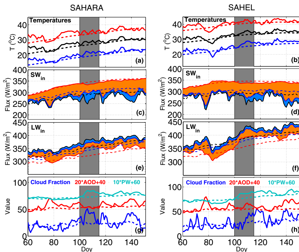
Fig. 2 Springtime time series of a, b T_{min} (blue), T_{avg} (black) and T_{max} (red); c, d daily-average SW_{in} (black), clear-sky SW_{in}^{clear} (blue), clear-sky SW_{in}^{clean} (red); blue shading therefore corresponds to the Cloud Radiative Effect and orange shading to the Aerosol Radiative Effect (see Sect. 4.1 for more details); e, f same as c, d for incoming long-
