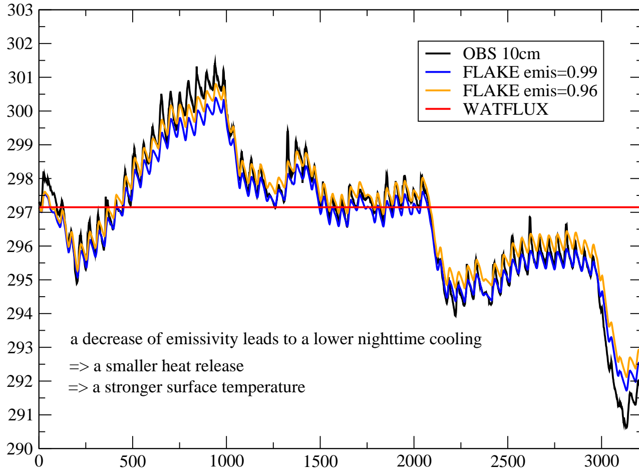
B5 : sensitivity to emissivity
