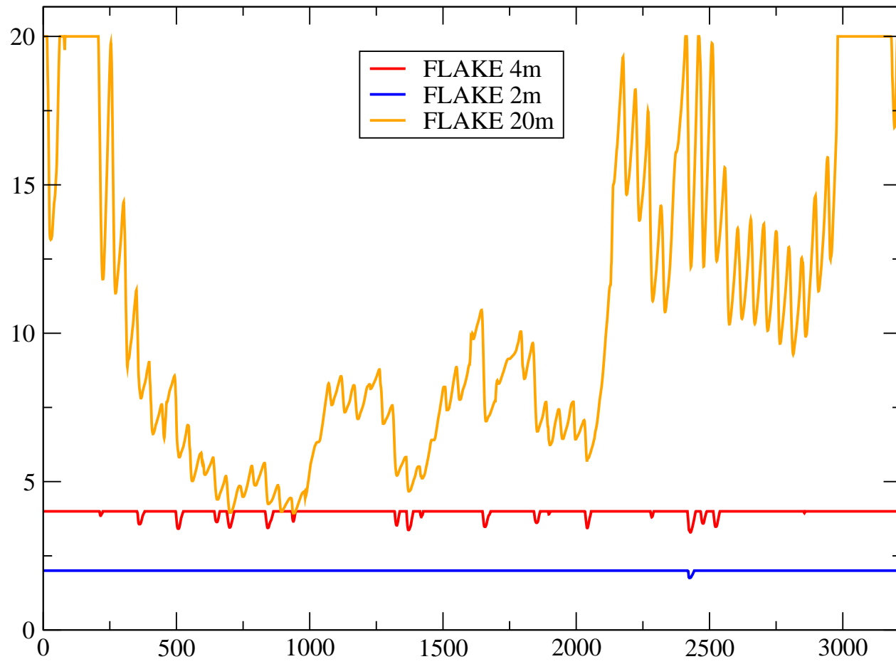
B8 : mixed layer depth
