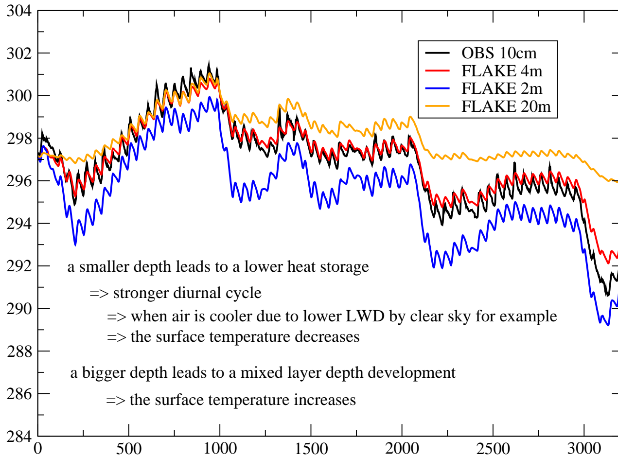
B7 : sensitivity to total depth
