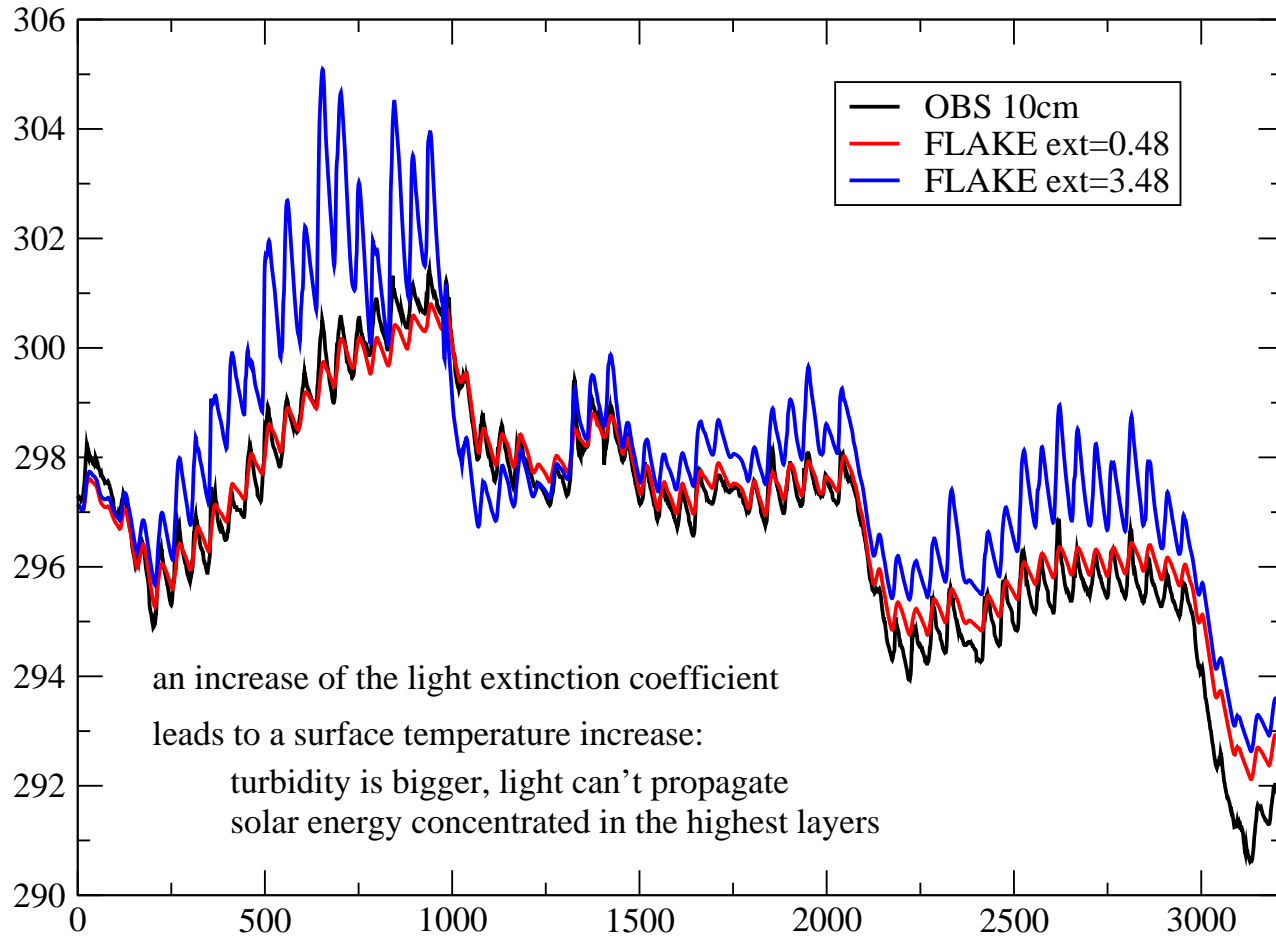
B10 : sensitivity to the extinction coefficient of light
