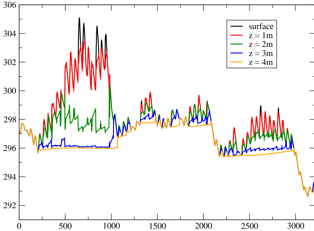
B12 : water temperature as a function of depth
