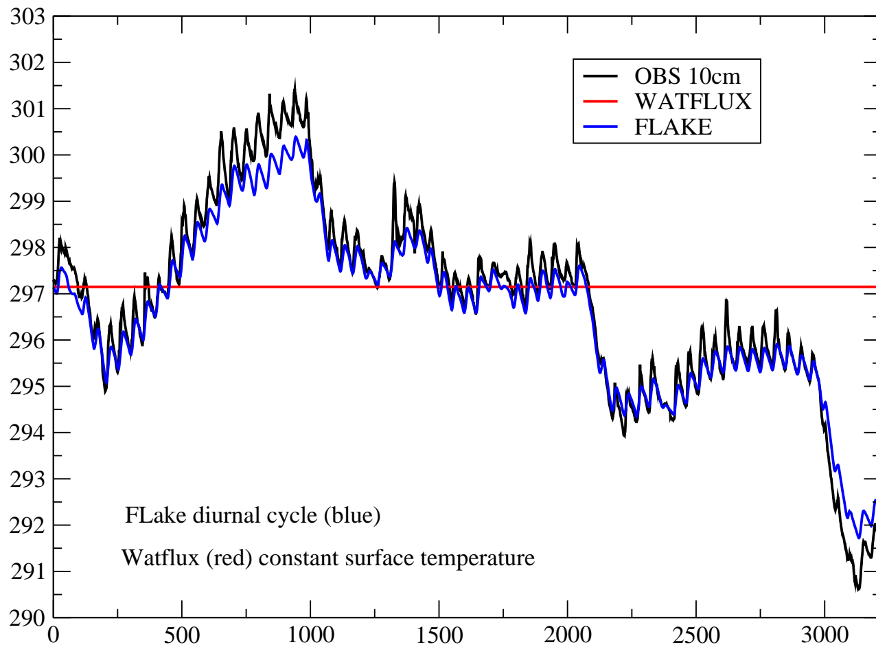
B3 : surface temperature
